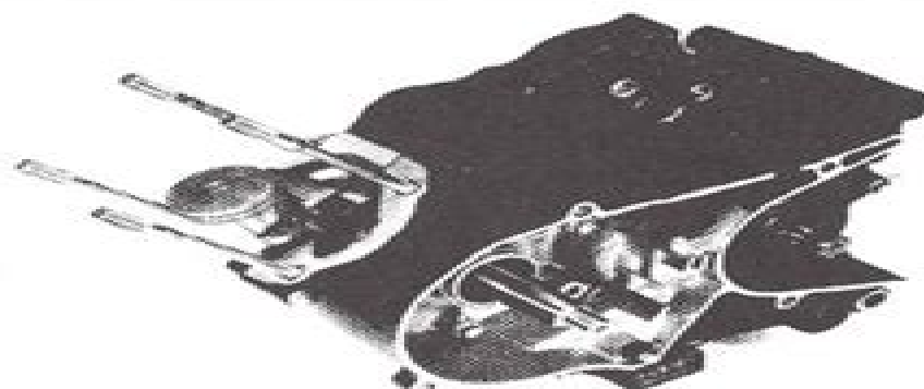
(1) CRANKCASE ASSEMBLY 07965-1660
