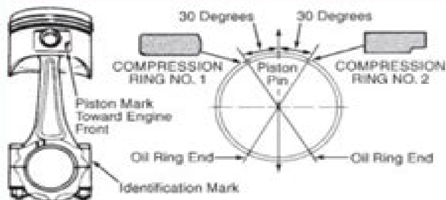
Fig. 28: Assembling Piston, Rod & Rings Courtesy of KIA MOTORS AMERICA, INC.
