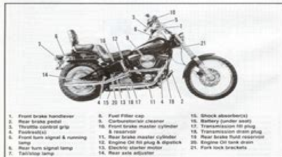
FIGURE 1-4. 1991 FXSTC - Right Side View
