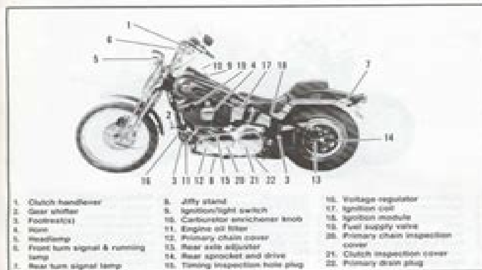
FIGURE 1-5. 1991 FXSTB - Left Side View
