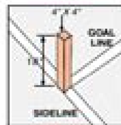
PYLON DETAIL
