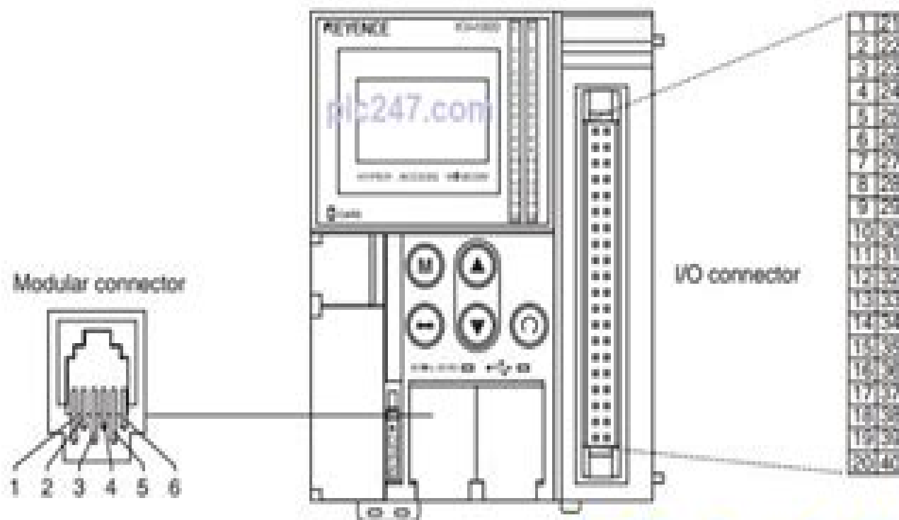
Modular connector
