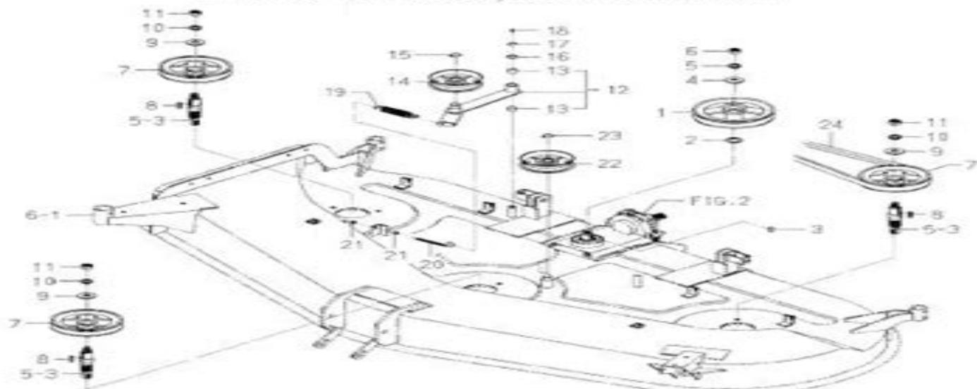
FIG. 3 PULLEY,BELT SYSTEM
