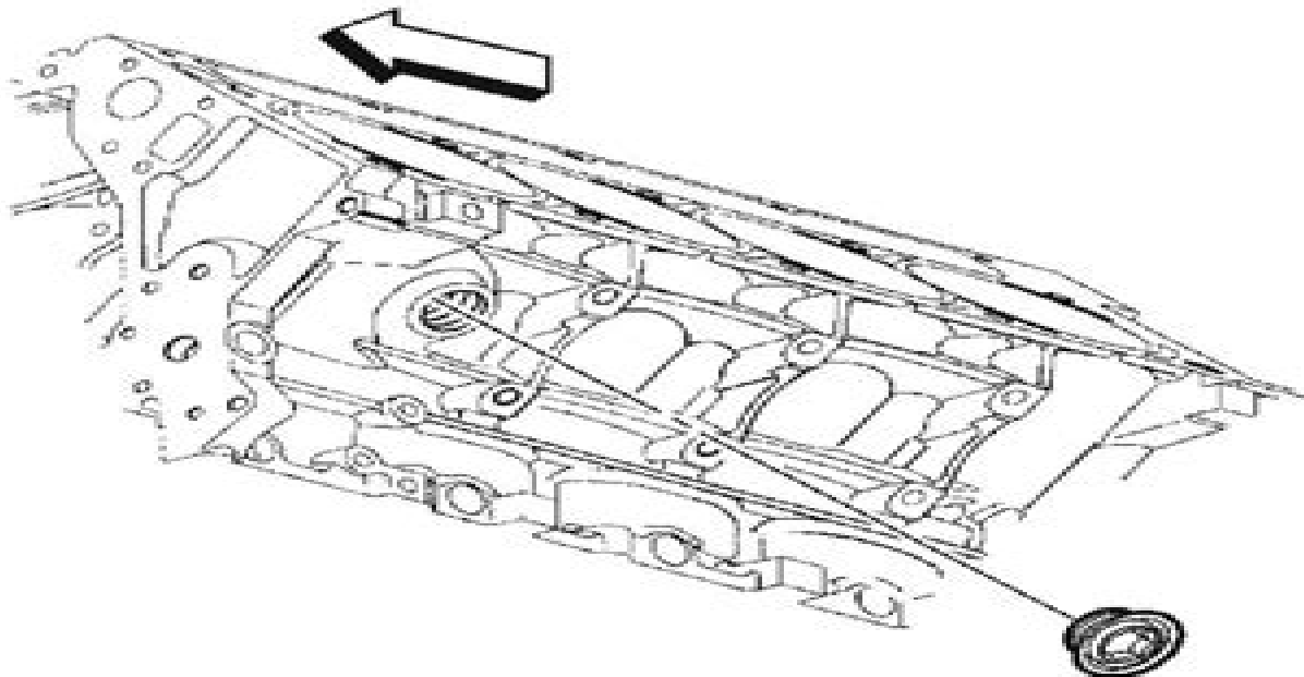
Fig. 2: View Of Engine Block Left Front Coolant Drain Hole Plug
