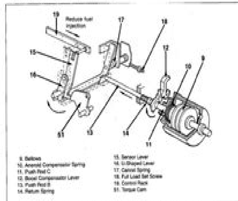
Figure 5. Link Motion when Aneroïd Compensator is Functioning
