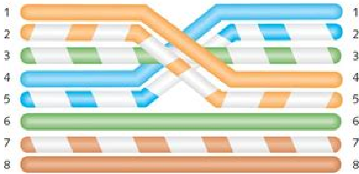
Figure 7-14 T1 crossover cable terminations Courtesy Course Technology/Cengage Learning
