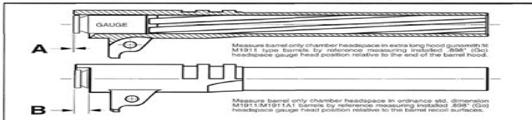
Figure 91- Illustrations by Heritage - VSP staff artist show barrel only chamber headspace checks in a long hood gunsmith fit M1911 type barrel at A, and in an ordnance standard (short hood) M1911A1 barrel, at B. See standard M1911/M1911A1 and NM barrel only chamber dimensional data in figure 89.
