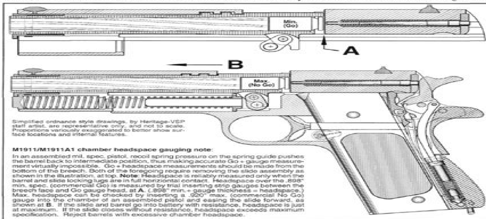
Figure 92- Ordnance style sectional illustration by Heritage - VSP staff artist, at top, shows a commercial minimum chamber (Go) headspace gauge installed in an M1911A1 slide assembly. The sectional illustration below depicts an M1911A1 pistol with excessive chamber headspace- as evidenced by the fact that, in this example, chamber length permitted the slide to close on a .920" maximum chamber (No Go) headspace gauge.
