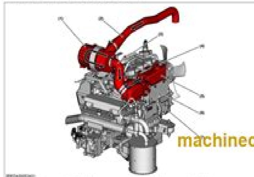
MECHANISM (1) Engine air cleaner (2) Intake air duct (3) Intake manifold (4) Throttle body (5) Engine (6) Air filter
