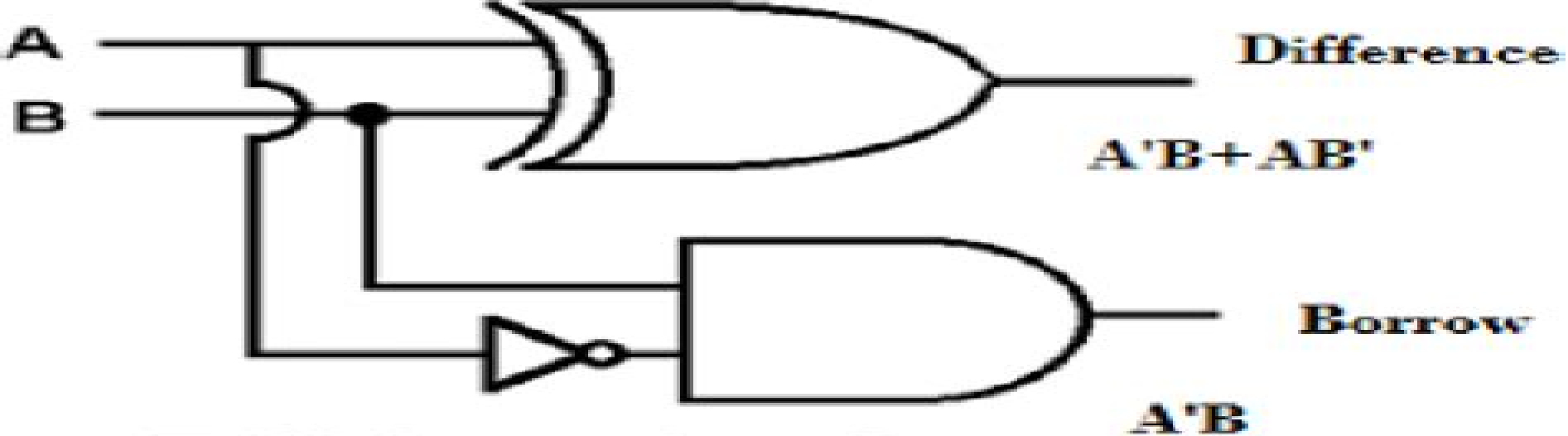
Half Subtractor Logic Diagram
