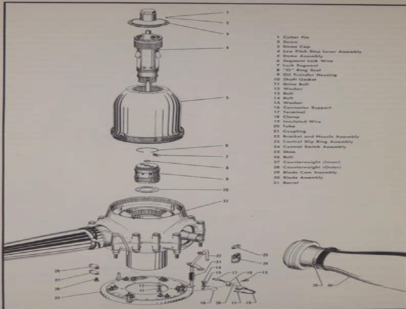
Figure 2-1. Model 43E60-305 Propeller Assembly
