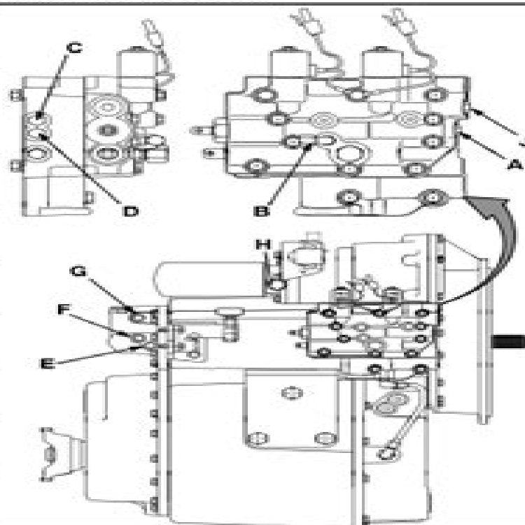
FIGURE 38. TRANSMISSION PRESSURES
