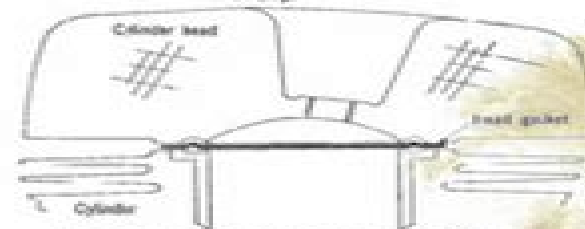
Fig. 6-1-2 Installing cylinder head gasket
