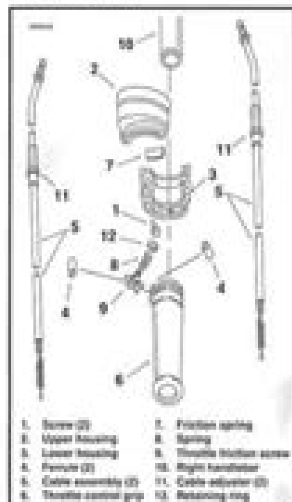
Figure 2-78. Throttle Control - Right Handlebar
