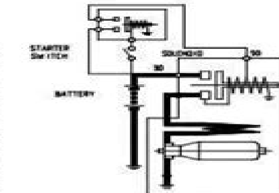
CONNECTING DIAGRAM RELAY
