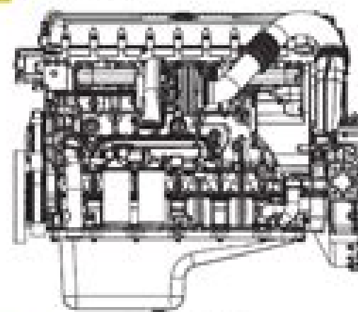
Figure 1: C13 TurboCompound 1200 (1000)
