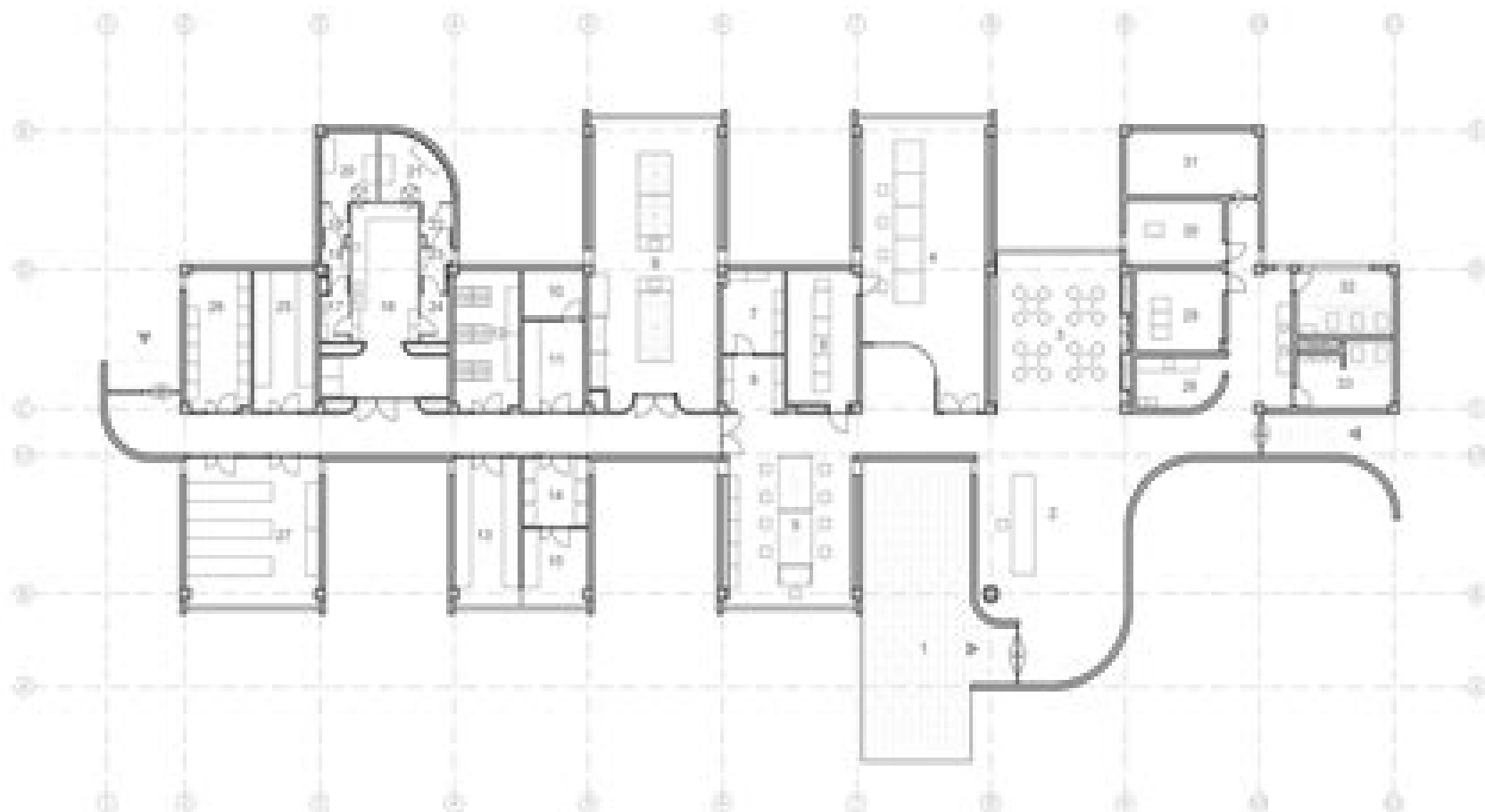
FLOOR PLAN 15
