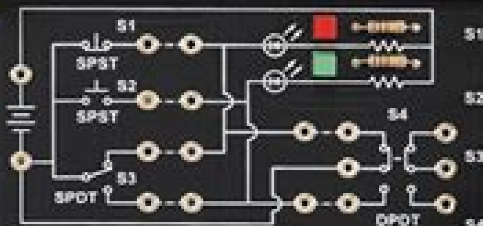
SWITCHES
