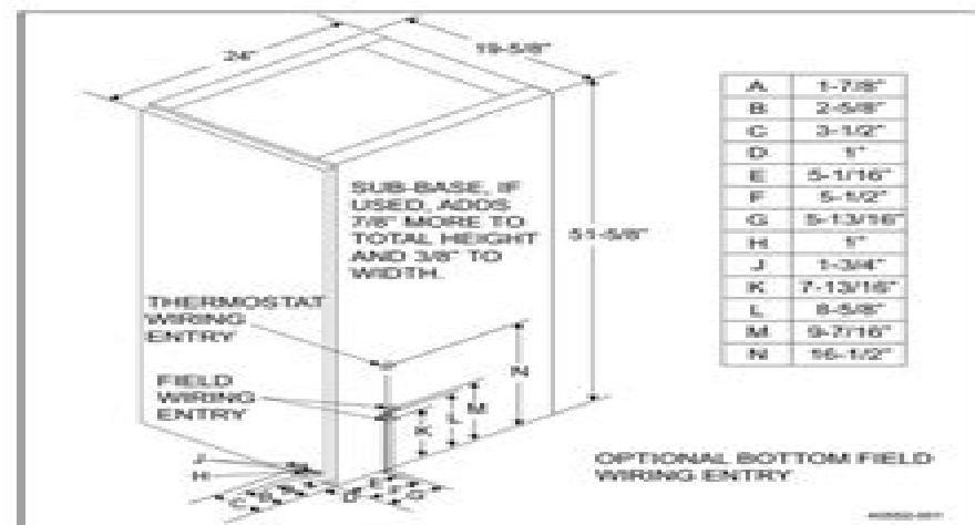
FIGURE 1: Furnace Dimensions
