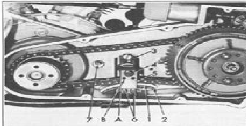
Figure 2-1. Adjusting Front Chain
