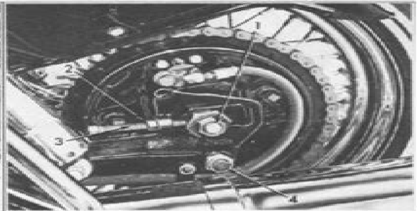
Figure 2-2. Adjusting Rear Chain (1972 and Earlier)
