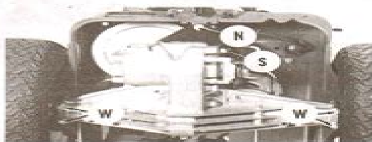
Fig. JD33—Unscrew nut (N), support screw (S) and outer screws (W) to lower or remove transaxle. See text.
