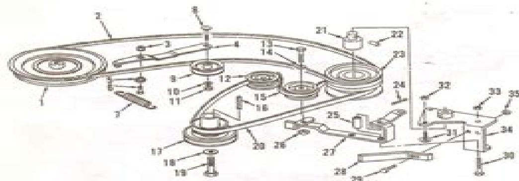
Fig. JD31—Exploded view of drive system.
