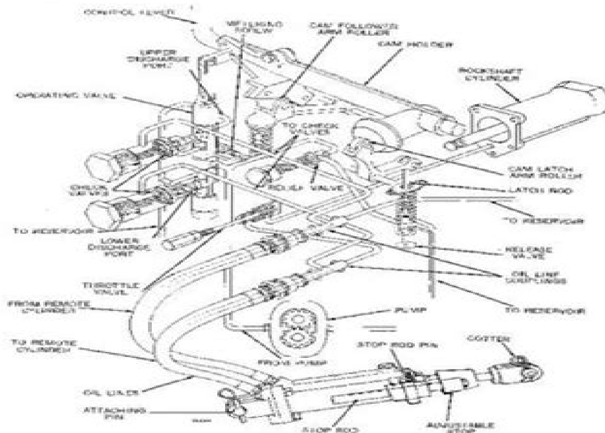
Figure 20-19-1—Orientation Diagram
