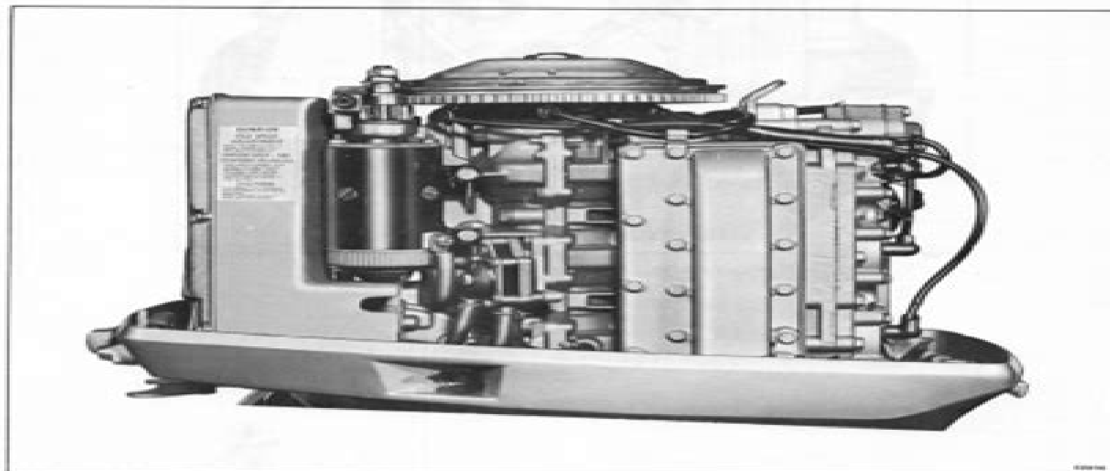
Figure 5-39. Port Side, Wiring and Clamps
