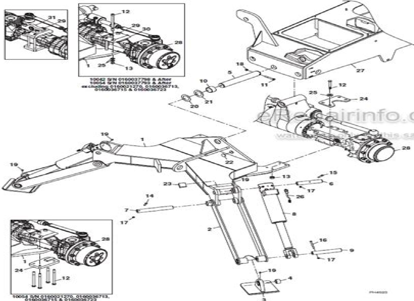
Figure 1-3 Outrigger Mounting
