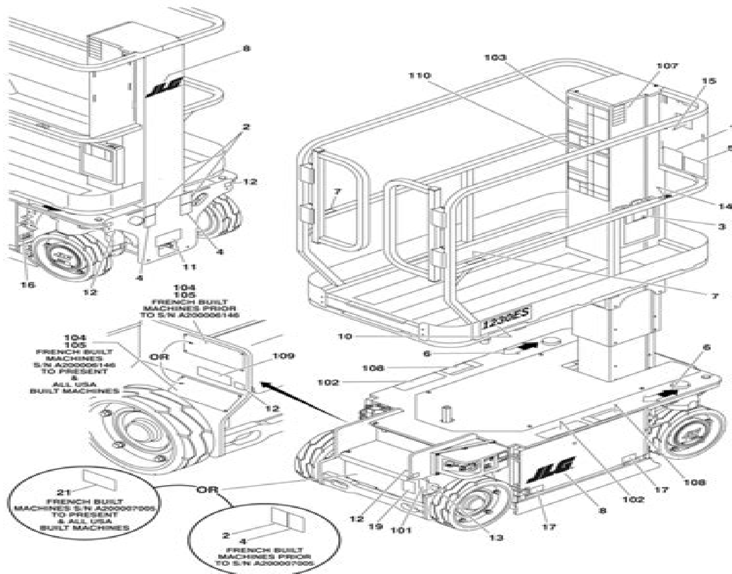
FIGURE 8-1. DECAL INSTALLATION
