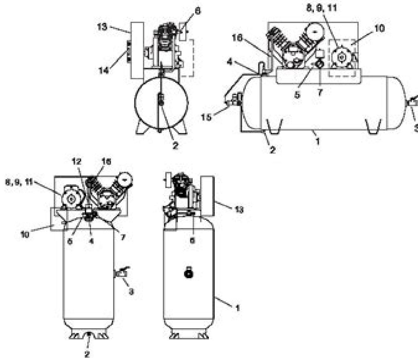
FIGURE 7. TYPICAL SIMPLEX RECEIVER MOUNTED ELECTRIC PACKAGE.
