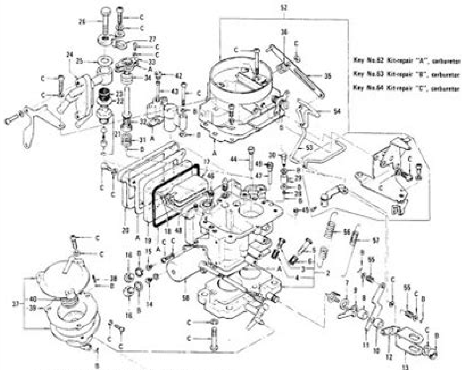
Carburetor (Hitachi-Daf 328-6) (L16 Manual)
