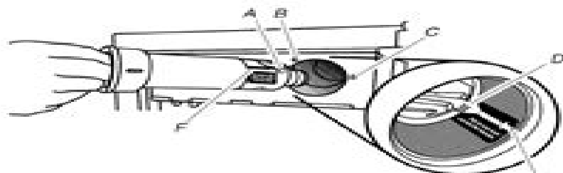
A. Alignment pin B. Unlocked symbol C. Locked symbol D. Cutout notch inside control housing E. Arrow pointing to cutout notch F. Arrow pointing to alignment pin
