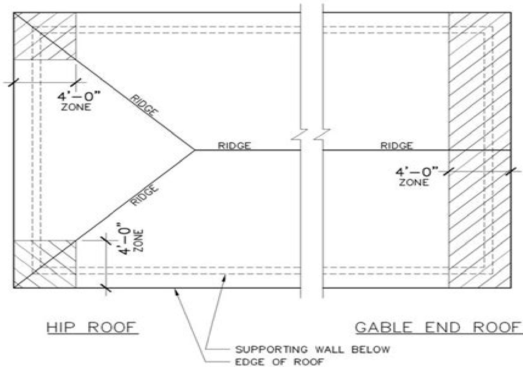
TYPICAL PLAN VIEW FOR ROOF N.T.S.
