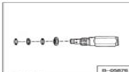
Fig. 2-25a Anti-Cavitation Valve
