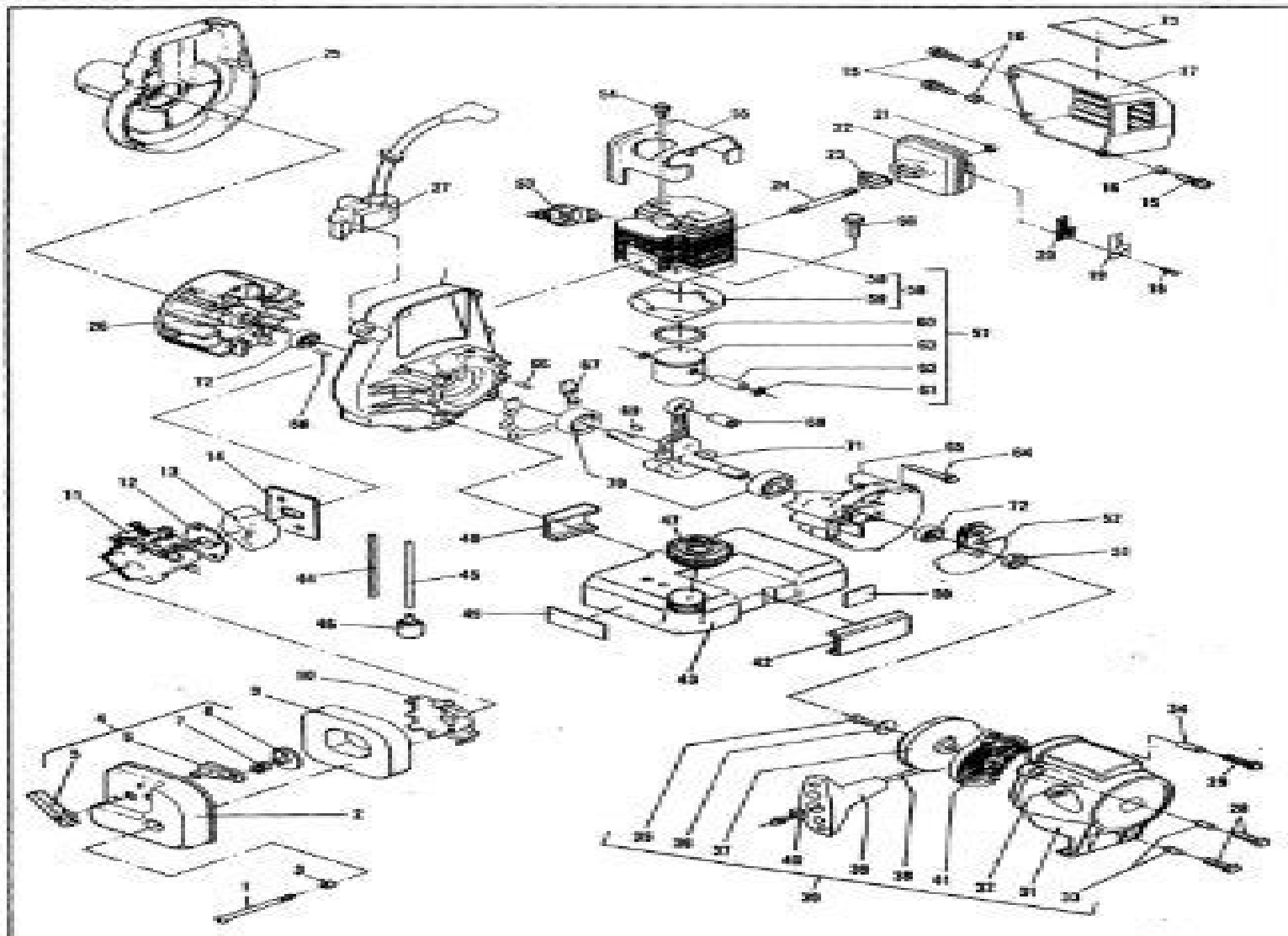
Figure 1 ENGINE ASSEMBLY
