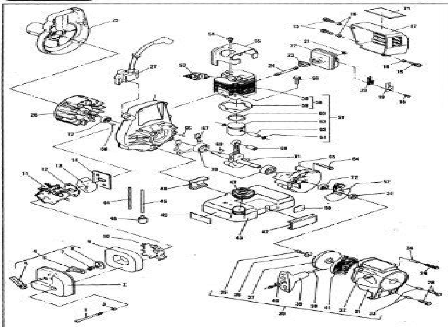
Figure 1 ENGINE ASSEMBLY
