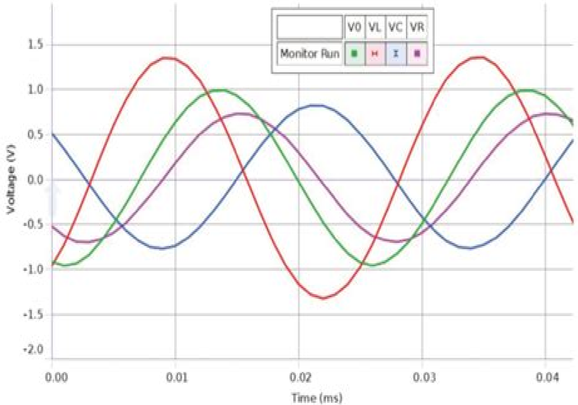
LRC Series Circuit above Resonance
