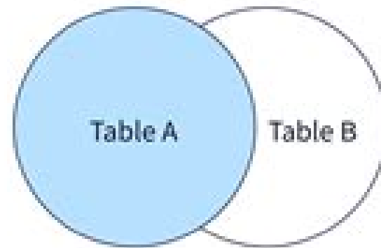
Left Join
