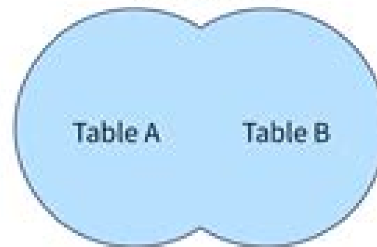
OUTER Join
