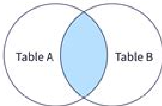
INNER Join
