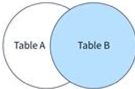
Right Join
