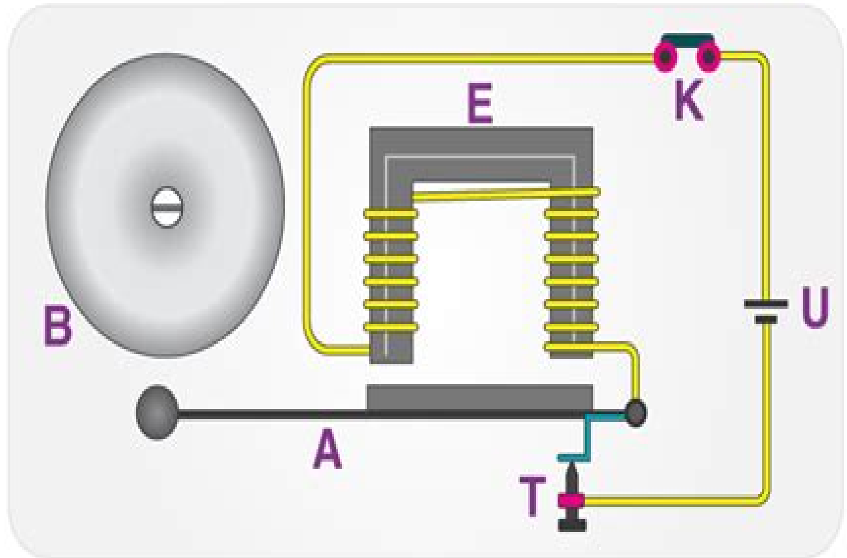
Electric Bell
