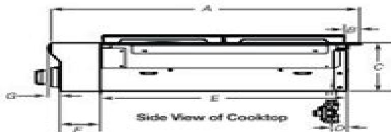
A. 27 1/4" (70.5 cm) B. 1 1/4" (3.2 cm) C. 7 1/4" (18.8 cm) D. Gas inlet is located 7 1/2" (19 cm) from the back of the cooktop burner base and 4 1/2" (11.4 cm) in from left-hand side of the cooktop burner base.
