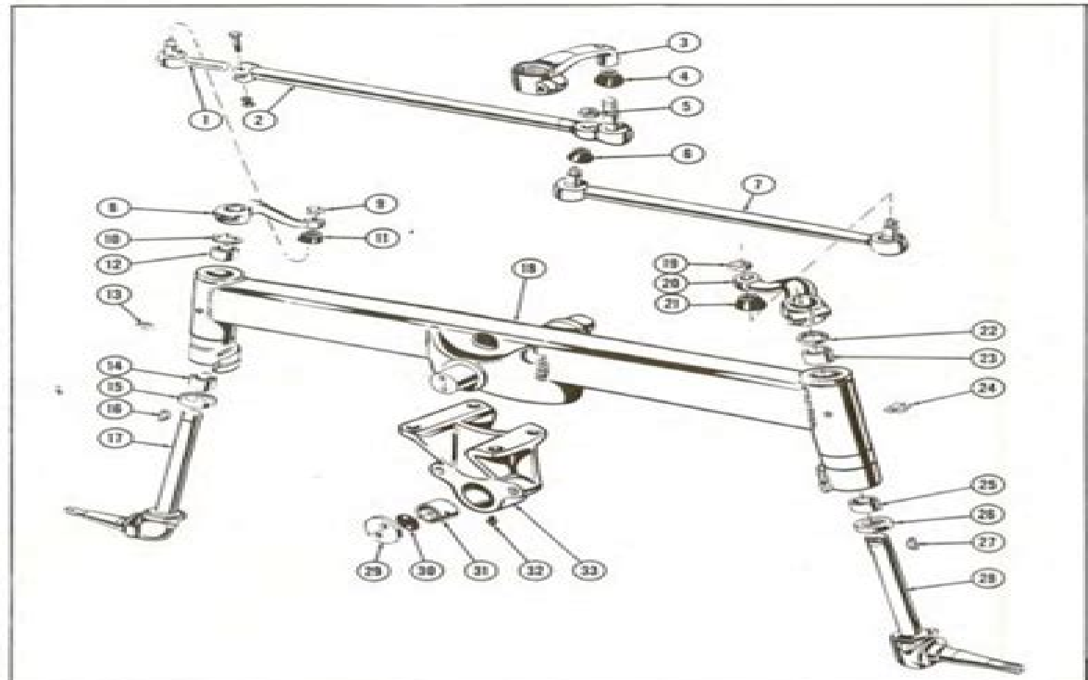
Fig. 4 - MF 50 Multi-Purpose Front Axle Assembly Nomenclature
