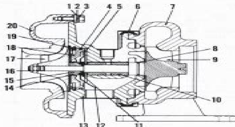
Fig. 87—Cross-section of Massey turbocharger showing location of parts.
