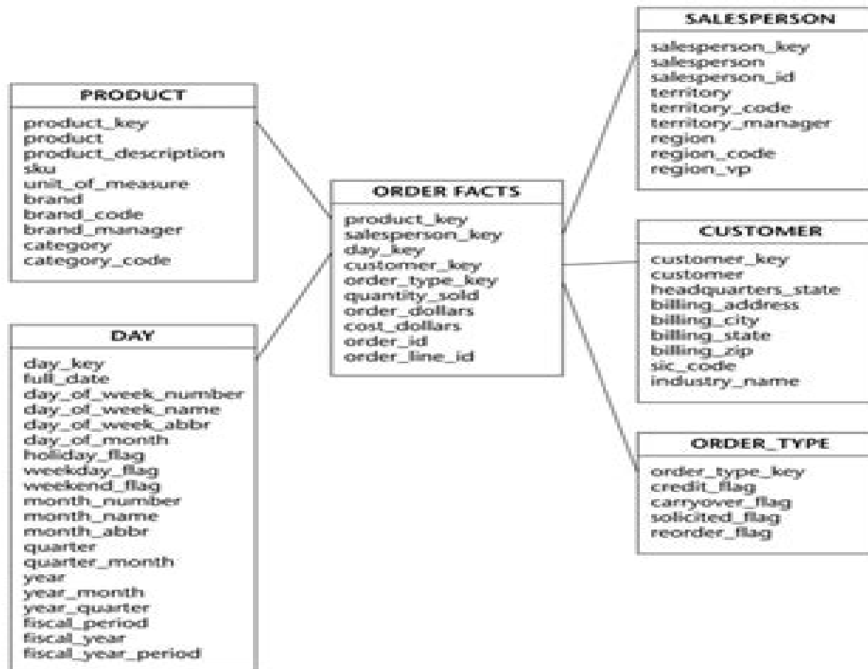
Figure 1.2 A star schema for the orders process.
