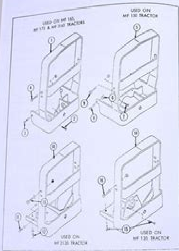
Fig. 1 - Mounting Bracket and Light - MF 130, MF 135, MF 210 and MF 210
