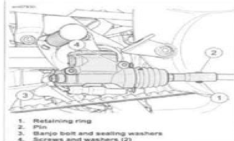
Figure 2-63. Rear Brake Master Cylinder
