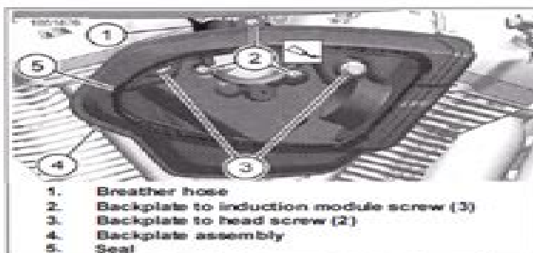
Figure 6-1. Breather Hose to Backplate Assembly
