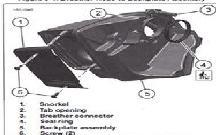
Figure 6-2. Backplate Assembly
