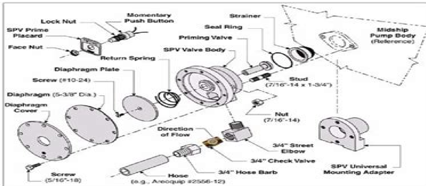
Figure 5-3: Hale SPV Parts Overview
