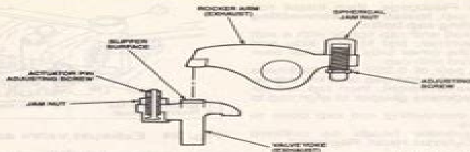
Fig. 25 J-TECH exhaust valve rocker arm & yoke
