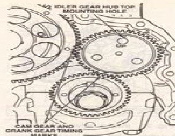
Fig. 26 Timing gear alignment marks
