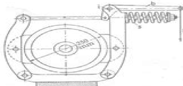
FIG. 2.1 Double-block crane brake.
