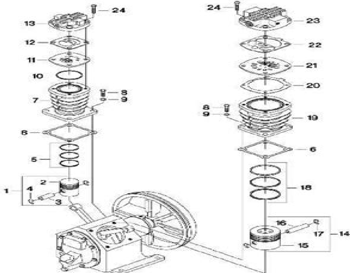
FIGURE 4. MODEL 3474 2-1/2" AIR COMPRESSOR.
