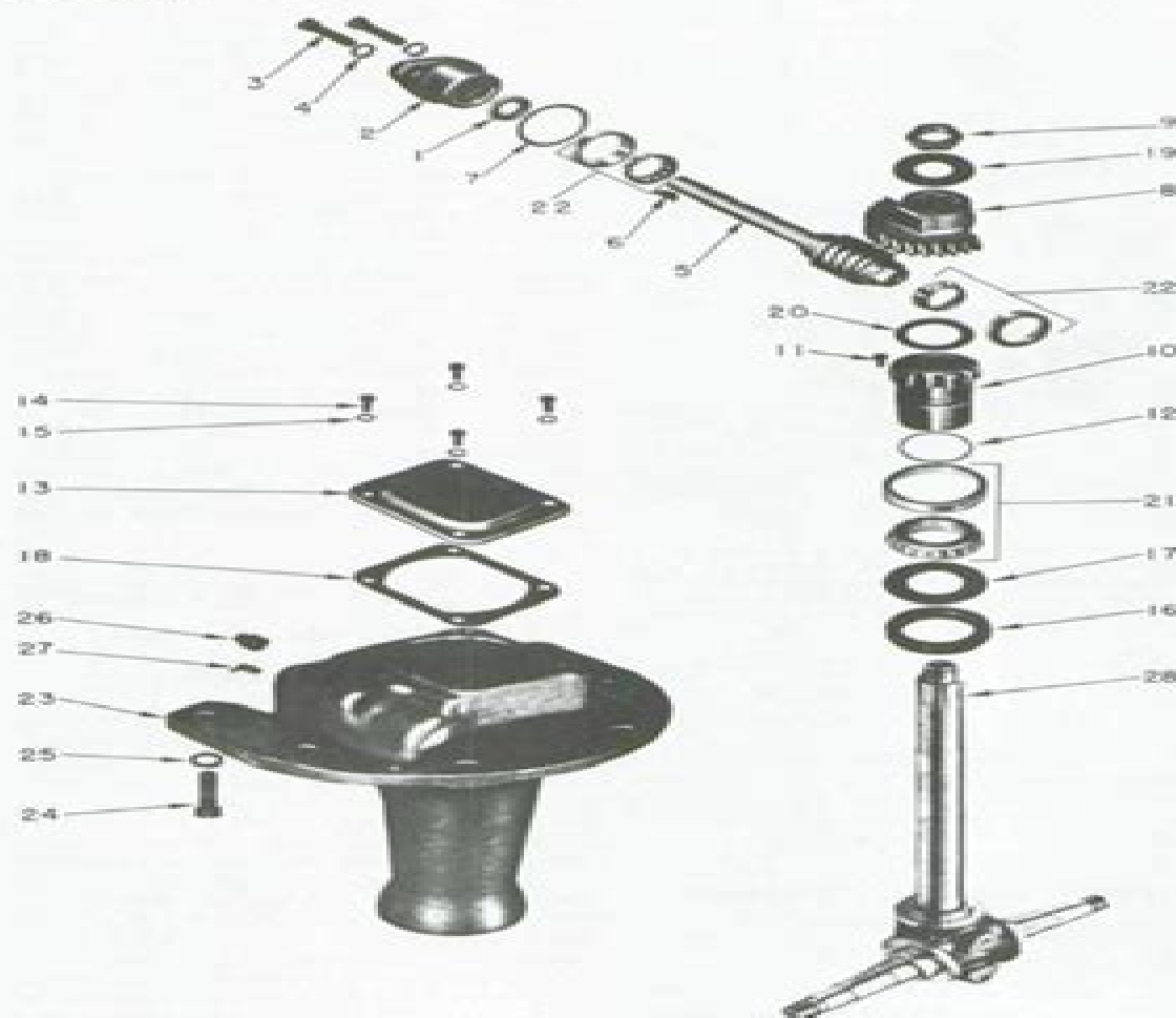
Fig. O8 — Exploded view of dual wheel tricycle front support and related parts as used on manual steering models. Refer to Fig. Q12 for front support for power steering models.
