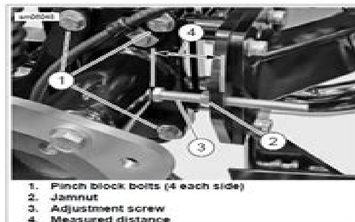
Figure 5-8. Adjust Axle
