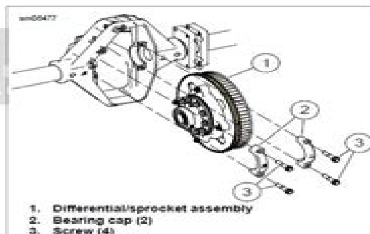
Figure 5-9. Differential and Sprocket Assembly
